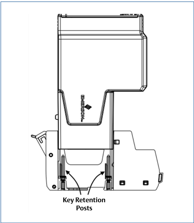
IS CHARM Standard Terminal Block.
