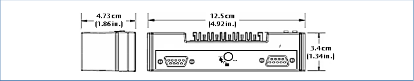
CHARM Baseplate Terminator Bottom.
