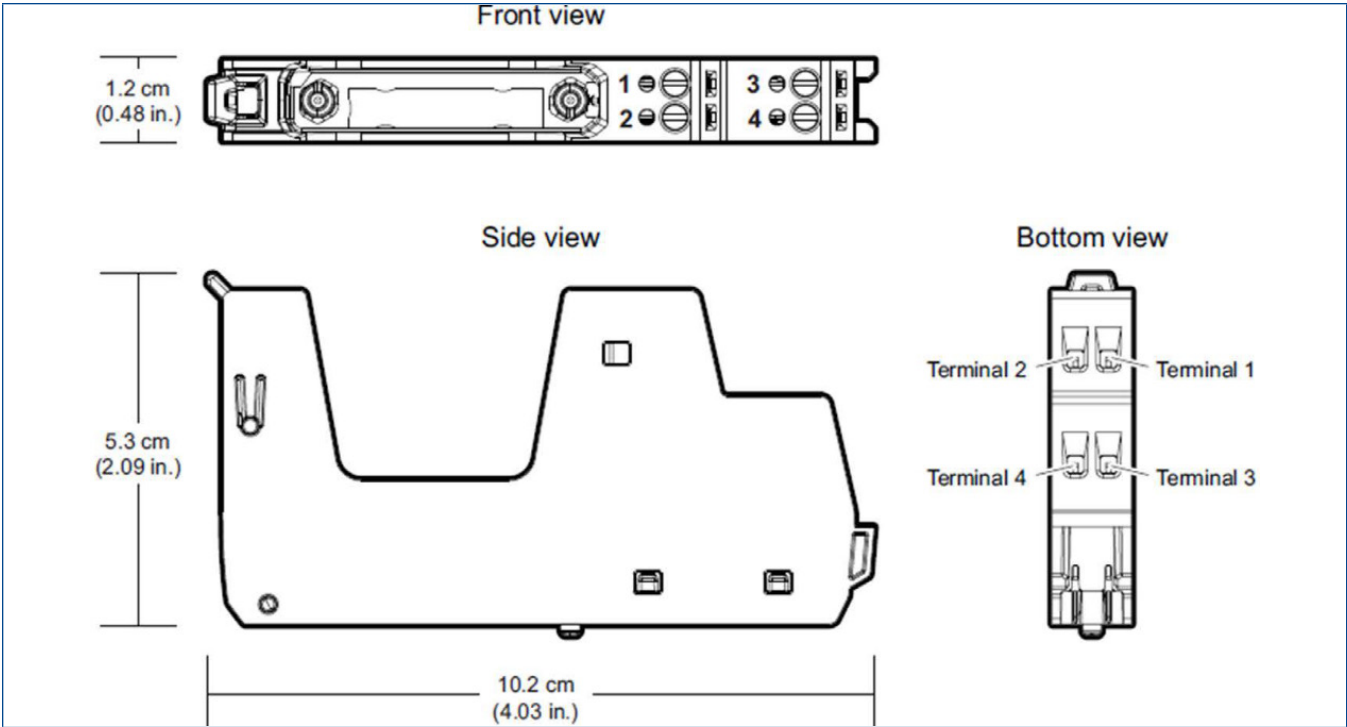
IS CHARM Terminal Block.
