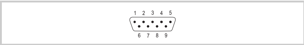
Abb. 13 RS232 interface (9-pin, D-Sub, male, UNC)
