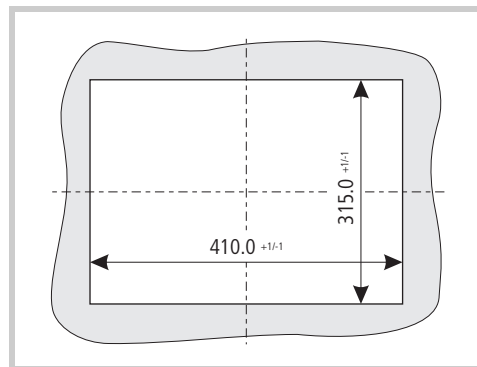
Abb. 21 Mounting cutout for 15" devices
