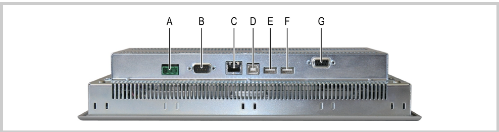
Abb. 7 Connector side of the device
