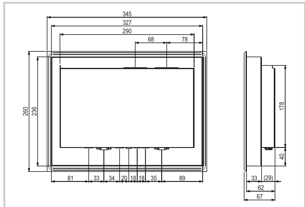
Abb. 30 Mechanical dimensions of the 10.4" devices in mm
