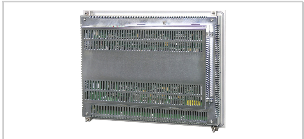
Abb. 24 10.4" and 12.1" devices with four retaining brackets (do not meet IP65 requirements)
