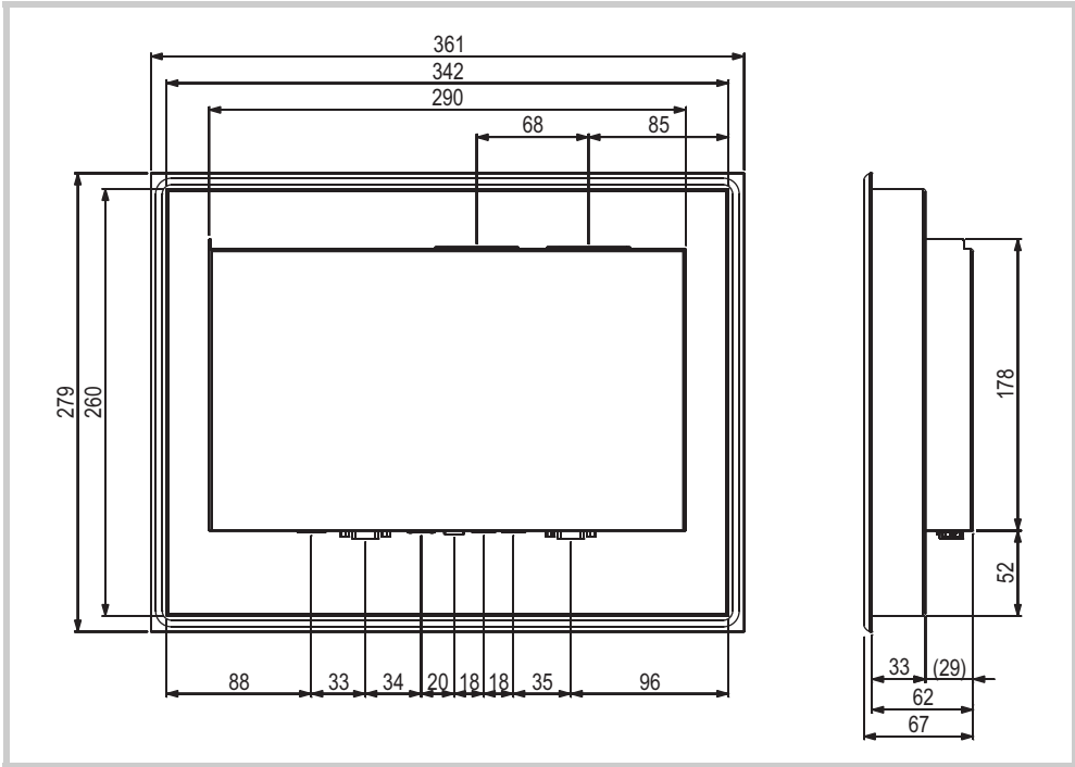
Abb. 31 Mechanical dimensions of the 12.1" devices in mm
